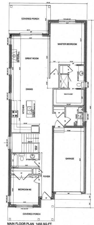
MAIN FLOOR PLAN 1455 SQ.FT.
