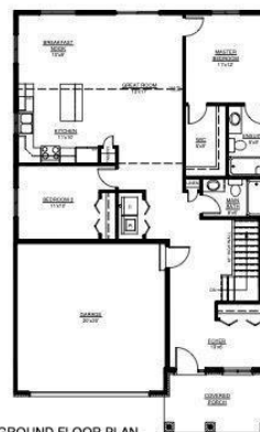
GROUND FLOOR PLAN 34'-8"X57'-0"
