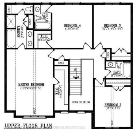
UPPER FLOOR PLAN 1453 SQ. FT. (PLUS 82 SQ. FT. OPEN)
