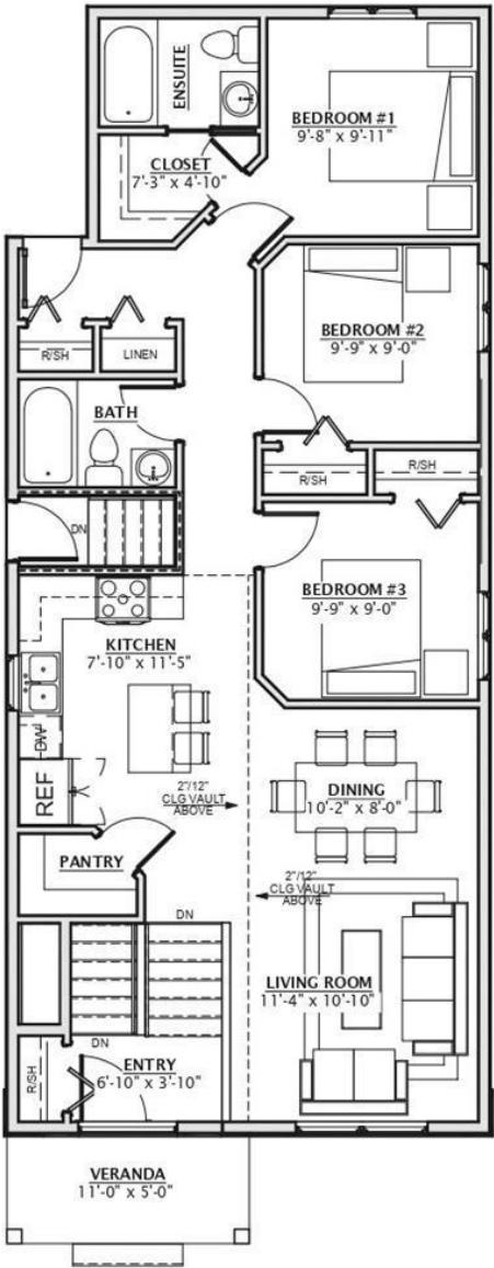
MAIN FLOOR 1091 ft 2
