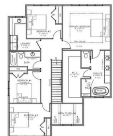
4 Bedroom Floor Plan
