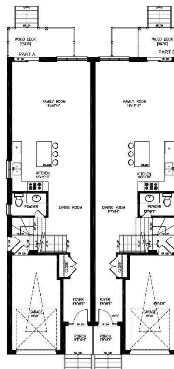
PROPOSED GROUND FLOOR PLAN SCALE: 1/4"=1'
