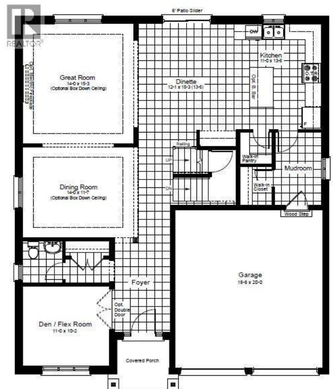
MAIN FLOOR Elevation A & B Licensed to CAOR
