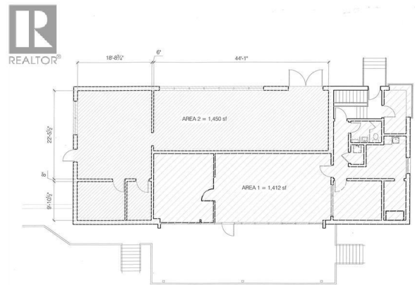
MAIN FLOOR PLAN SCALE: 3/32" = 1'-0"
