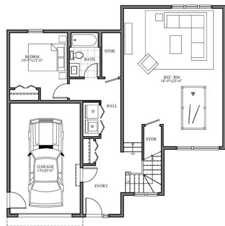
Grade Level Plan
